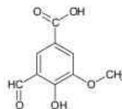
5-formylvanillic acid
