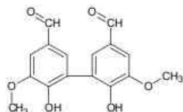
dehydrodivanillin
