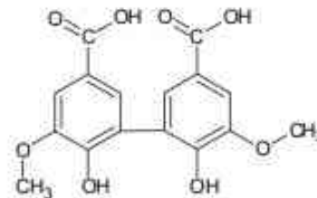
dehydrodivanillic acid
