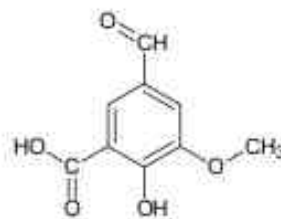
5-carboxyvanillin
