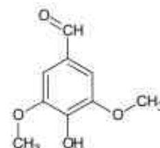
syringic aldehyde
