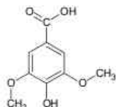
syringic acid
