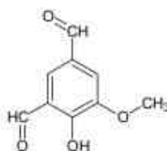
5-formylvanillin
