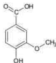
vanillic acid
